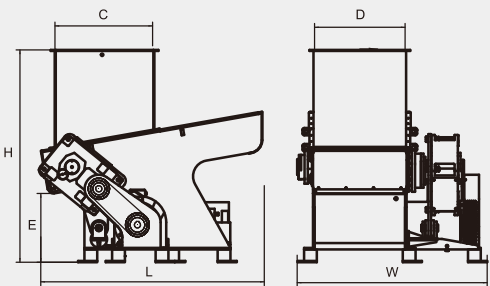
经济型单轴撕碎机 ECONOMICAL SINGLE-SHAFT SHREDDER
